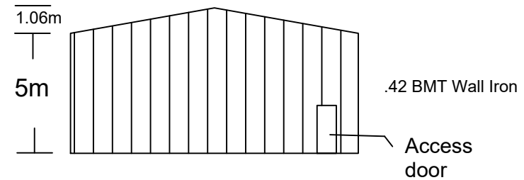
West Elevation
