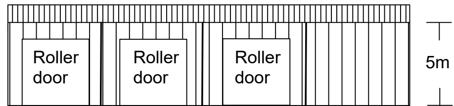
South Elevation
