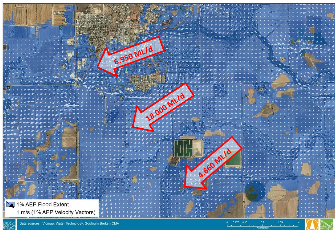
Figure 11-21 1% AEP peak flows at key flow paths across floodplain near Numurkah
