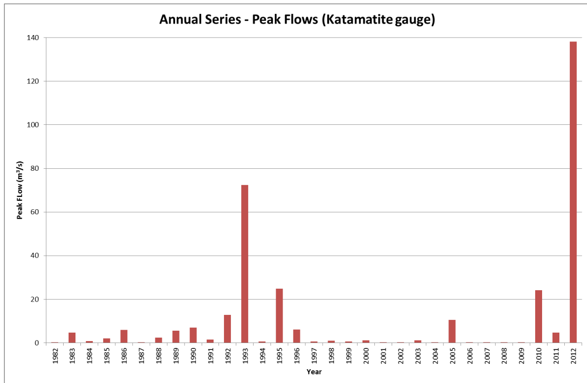
Figure 8-2 Annual series of peak flows at Boosey Creek at Katamatite gauge (404214)
