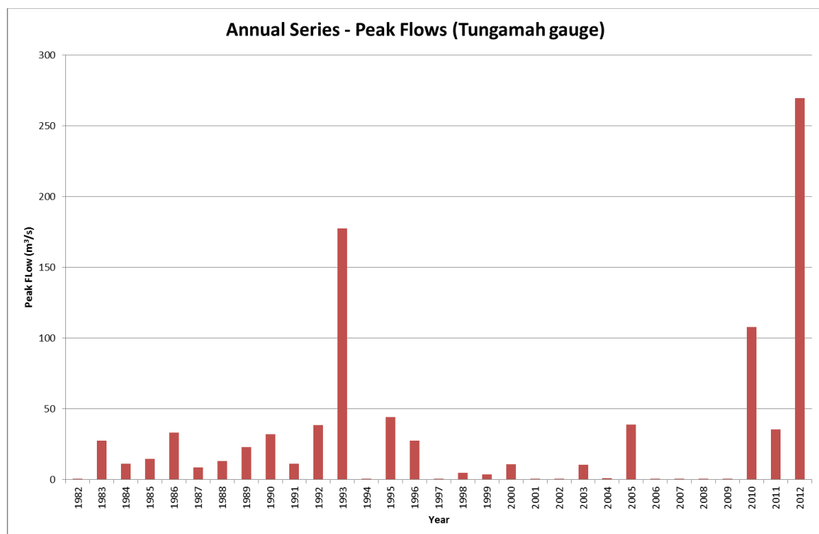
Figure 8-1 Annual series of peak flows at Boosey Creek at Tungamah gauge (404204)
