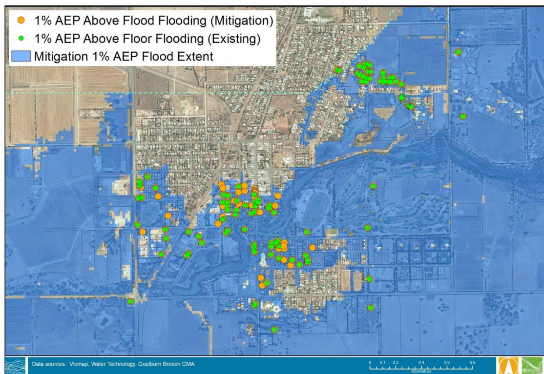
Figure 17-9 Comparison of buildings flooded above floor under mitigation scenario
