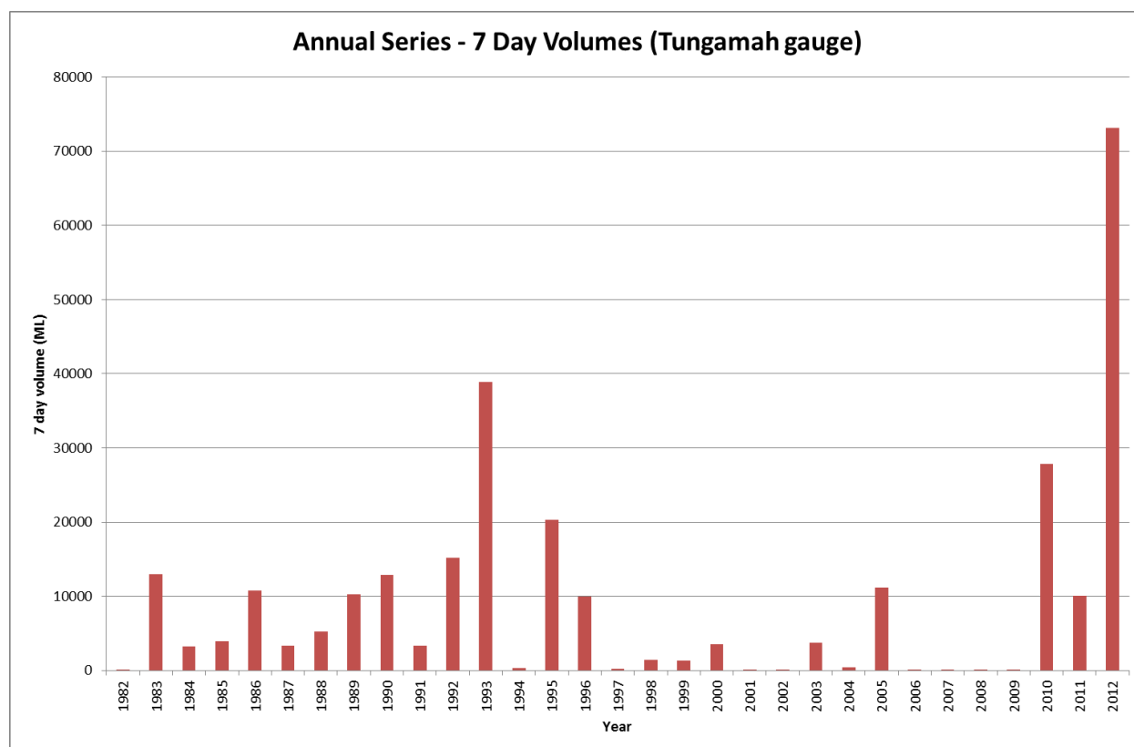
Figure 8-5 Annual series of 7 day volumes at Boosey Creek at Tungamah gauge (404204)
