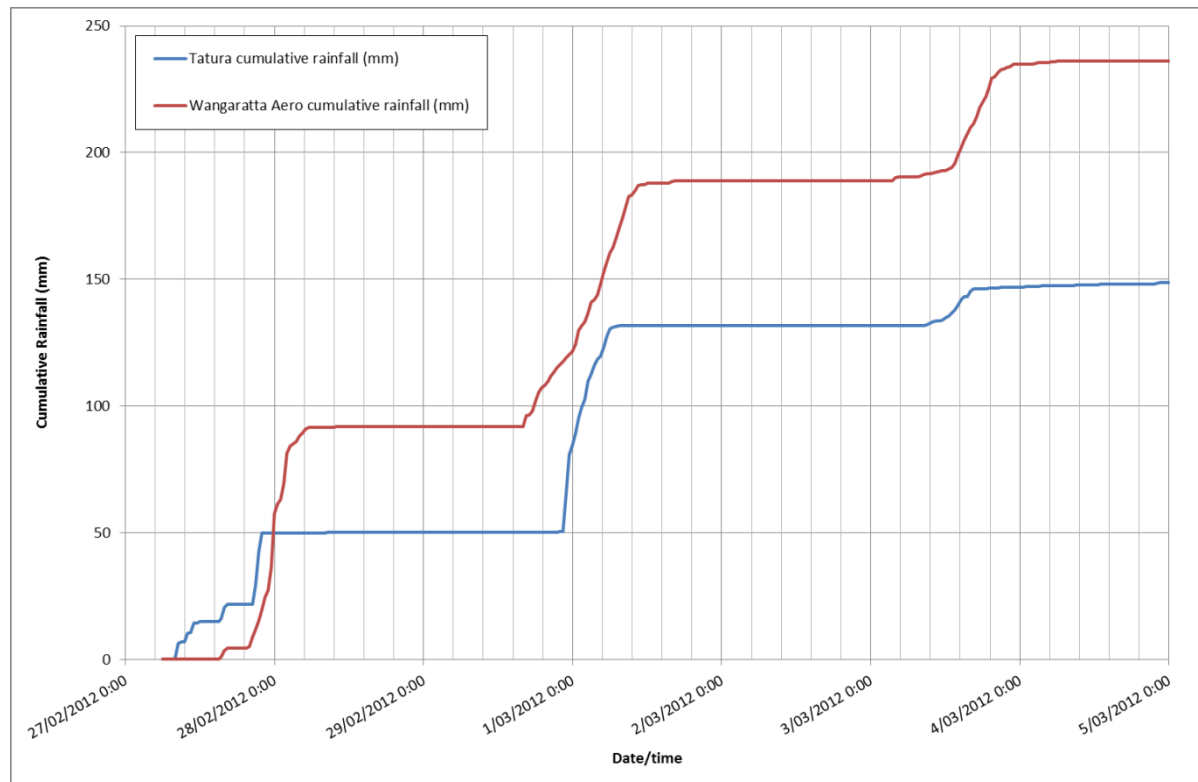
Figure 6-9 Observed temporal patterns at Tatura (81049) and Wangaratta Aero (81238) for the March 2012 event
