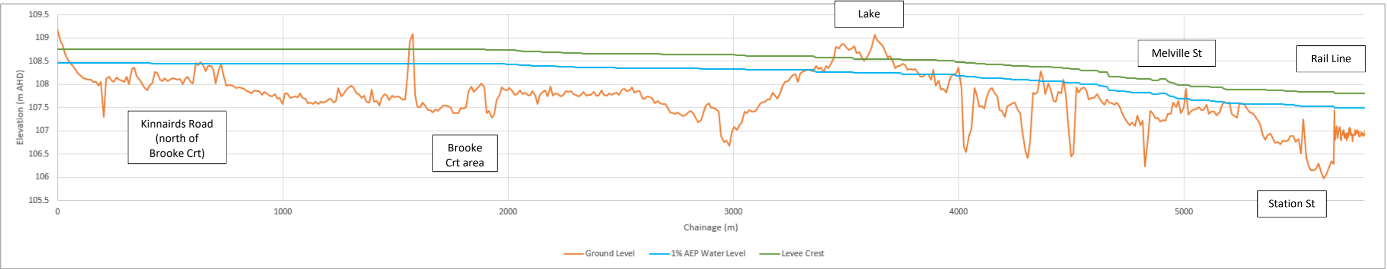
Figure 12-14 Long-section along northern levee alignment for Mitigation Package B
