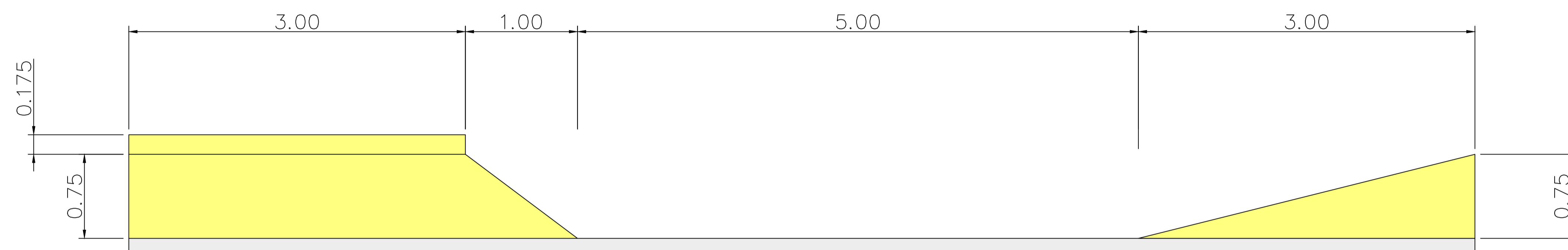
SECTION B-B
